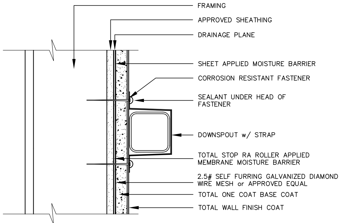
TODS-10 TYPICAL DOWNSPOUT ATTACHMENT
