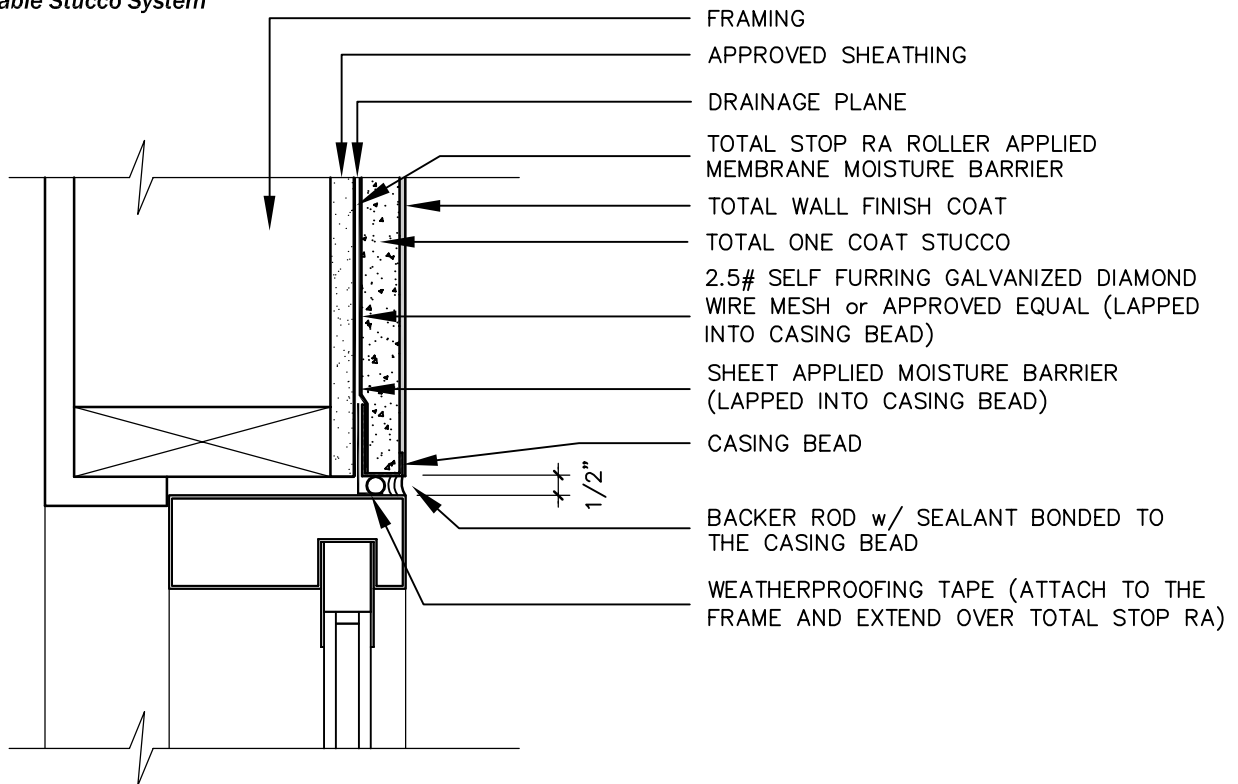
TODS-05.1 TYPICAL WINDOW/DOOR JAMB (FLUSH) - TOP VIEW
