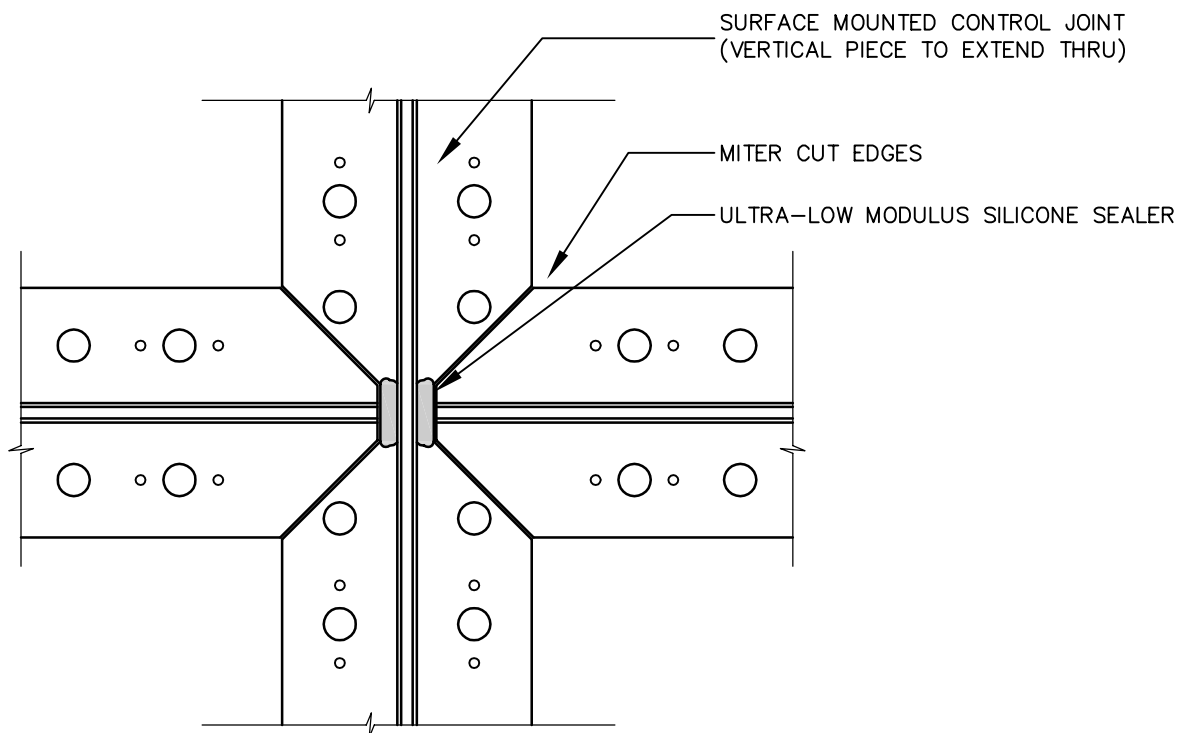
TODS-06.3 TYPICAL CONTROL JOINT - ELEVATION VIEW
