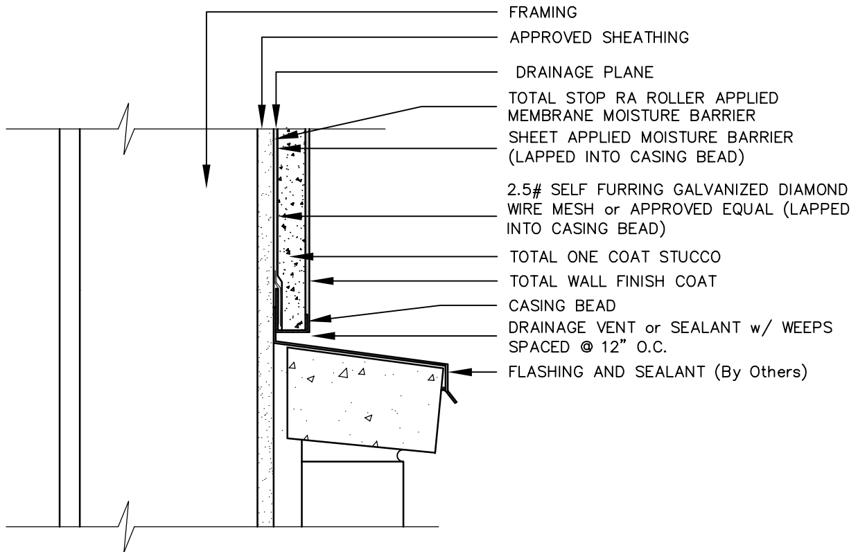
TODS-08.1 TYPICAL STUCCO @ MASONRY SILL
