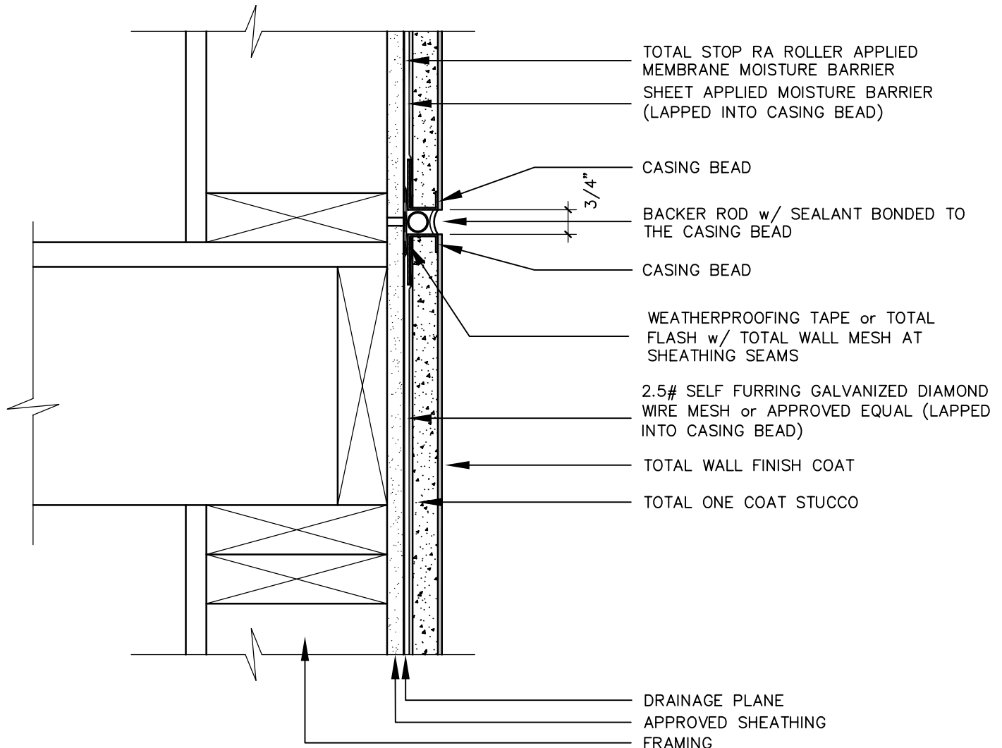
TODS-06.1 TYPICAL EXPANSION JOINT
