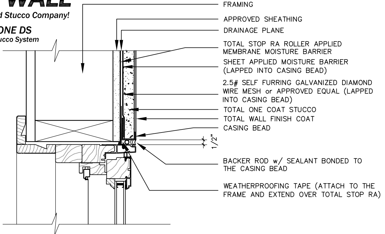
TODS-05.3 TYPICAL WINDOW/DOOR JAMB (FLUSH) - TOP VIEW
