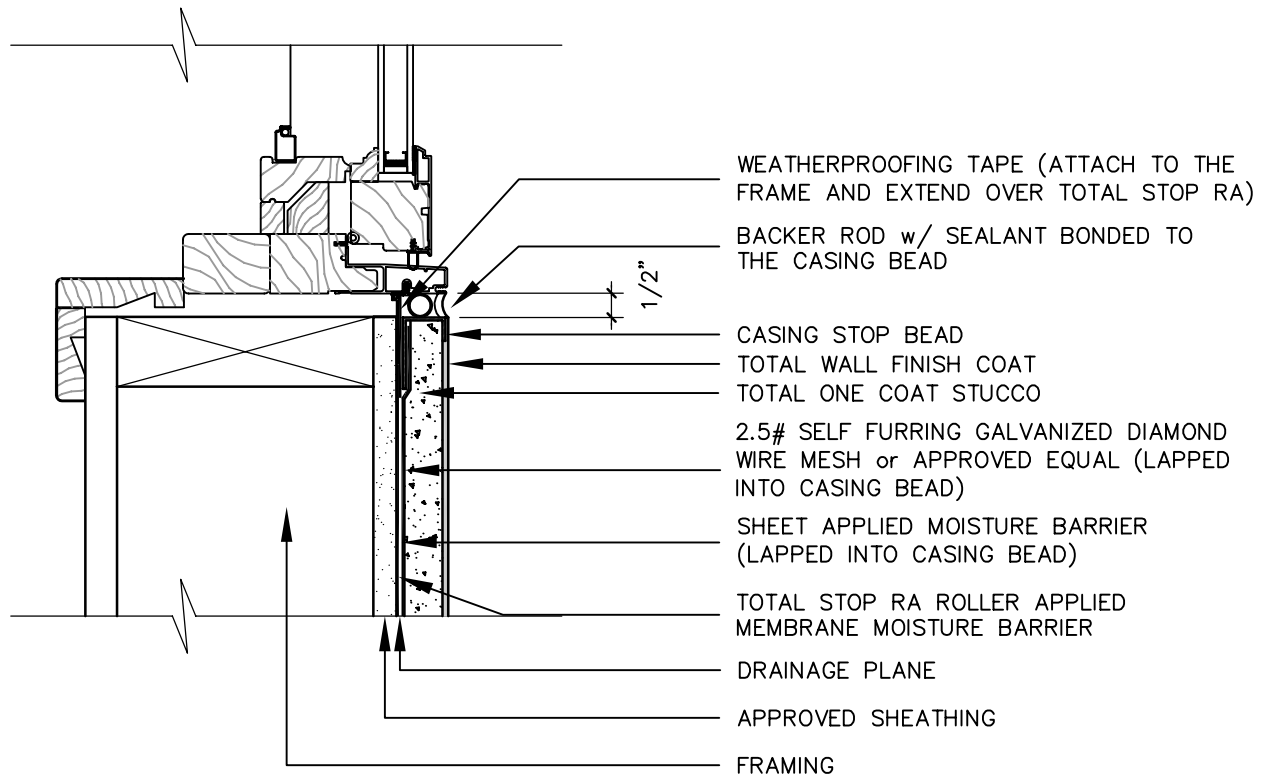
TODS-04.3 TYPICAL WINDOW SILL (FLUSH)
