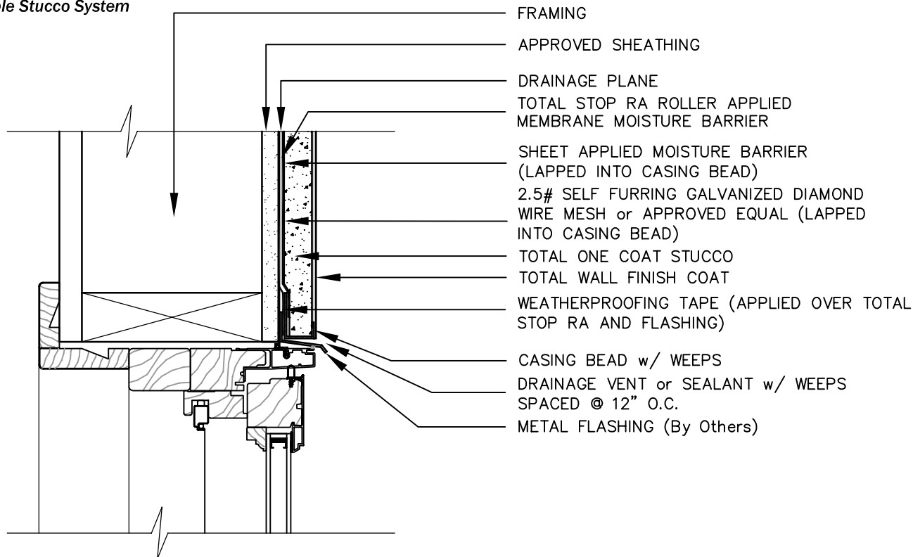
TODS-03.3 TYPICAL WINDOW/DOOR HEAD (FLUSH)
