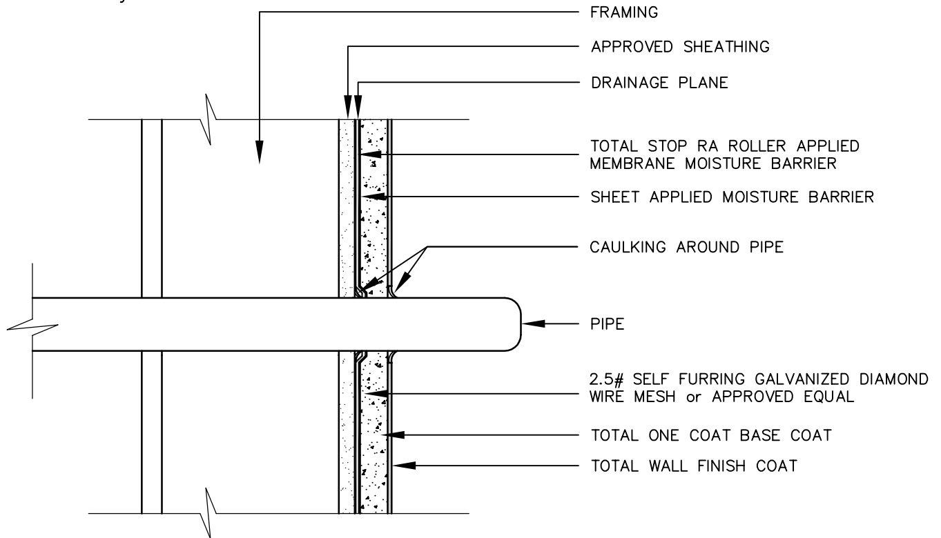
TODS-09 TYPICAL PIPE PENETRATION
