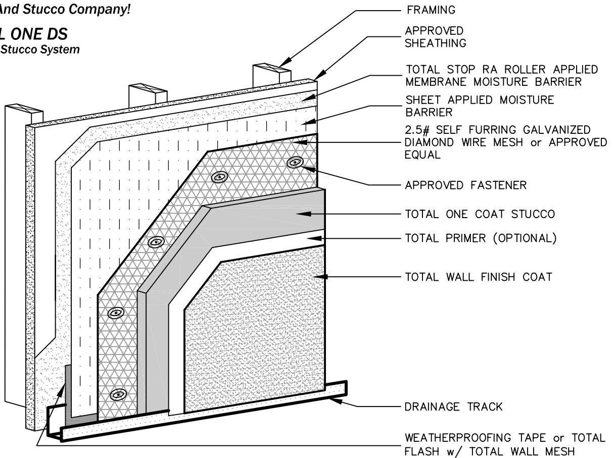
TODS-01 TYPICAL TOTAL ONE DRAINABLE STUCCO - ISOMETRIC
