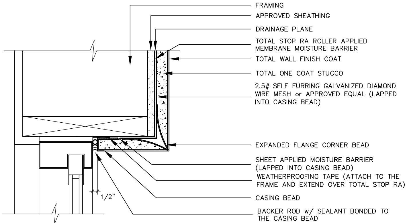
TODS-05.2 TYPICAL WINDOW/DOOR JAMB (RECESSED) - TOP VIEW
