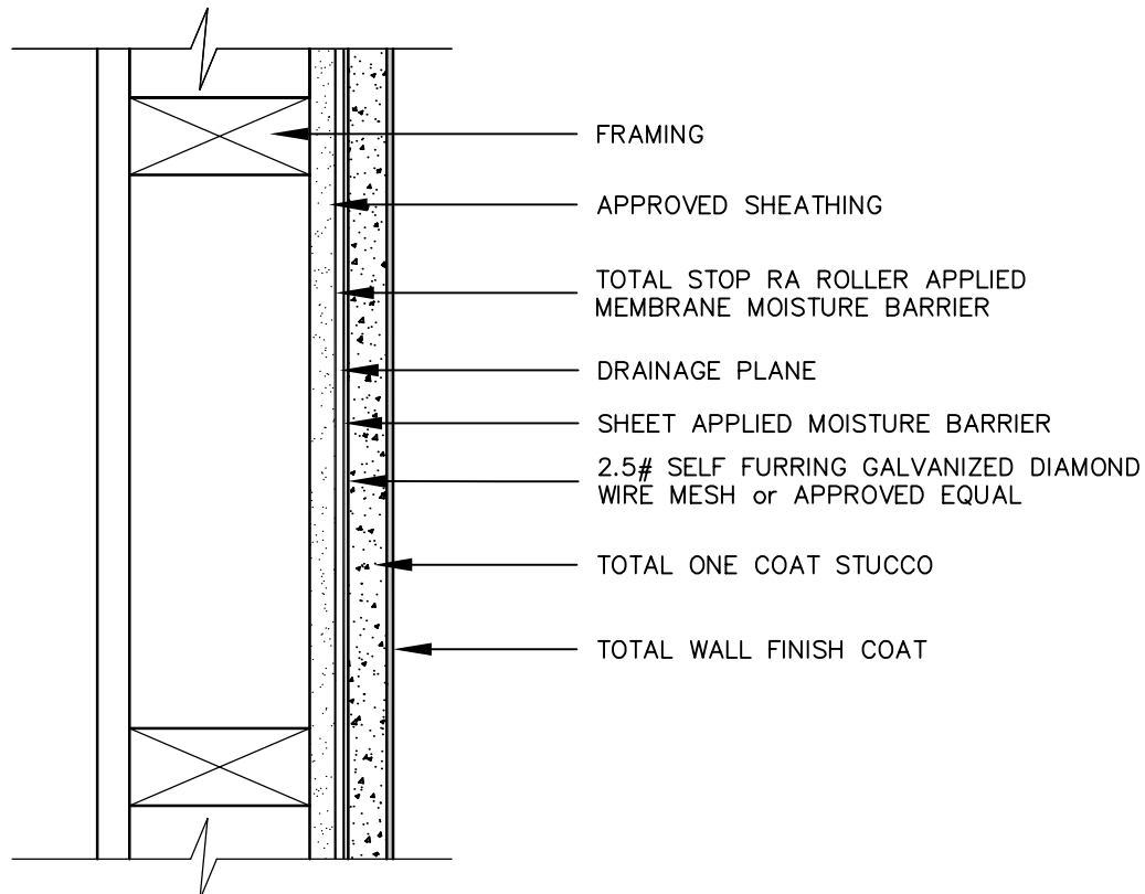
TODS-02 TYPICAL TOTAL ONE DRAINABLE STUCCO - PLAN VIEW
