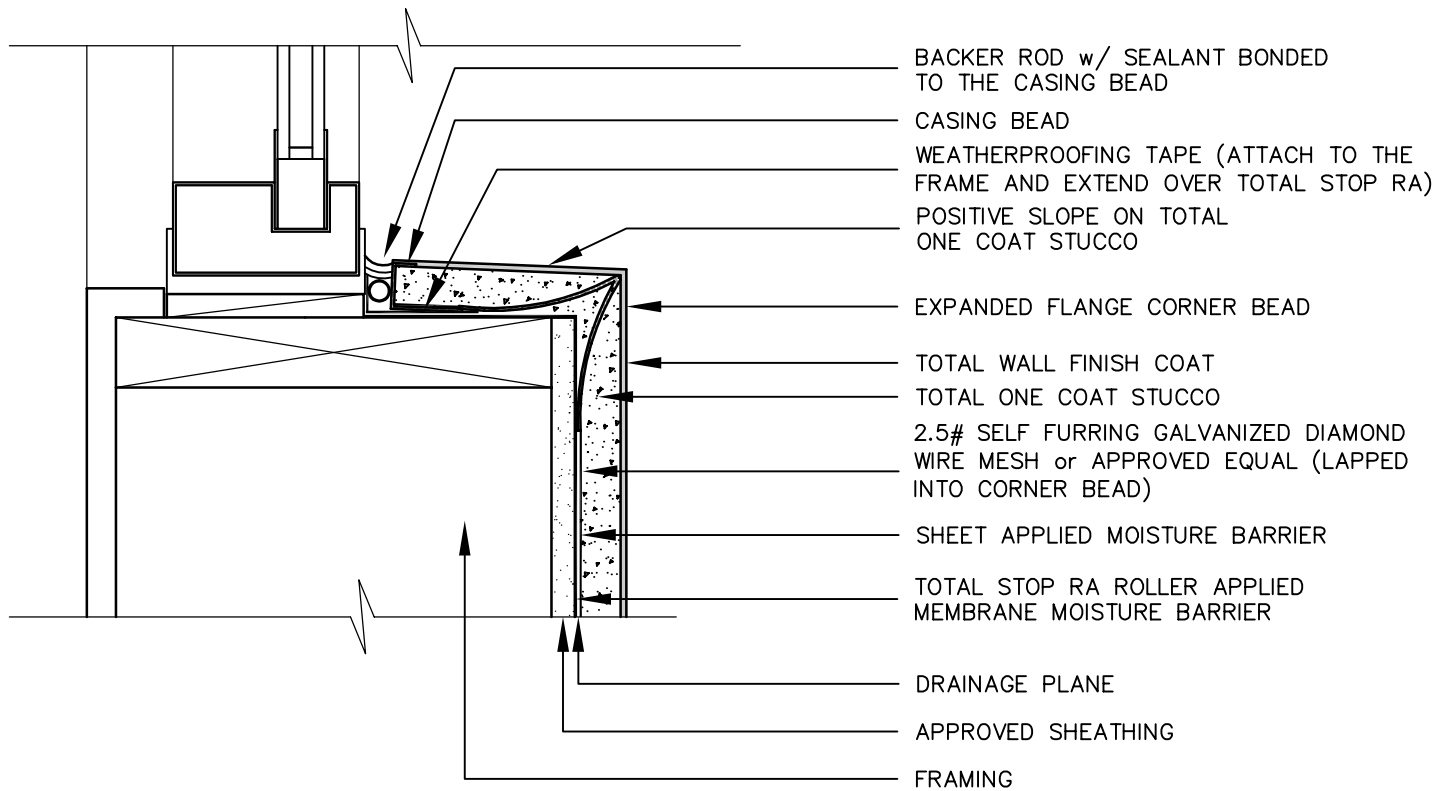
TODS-04.2 TYPICAL WINDOW SILL (RECESSED)
