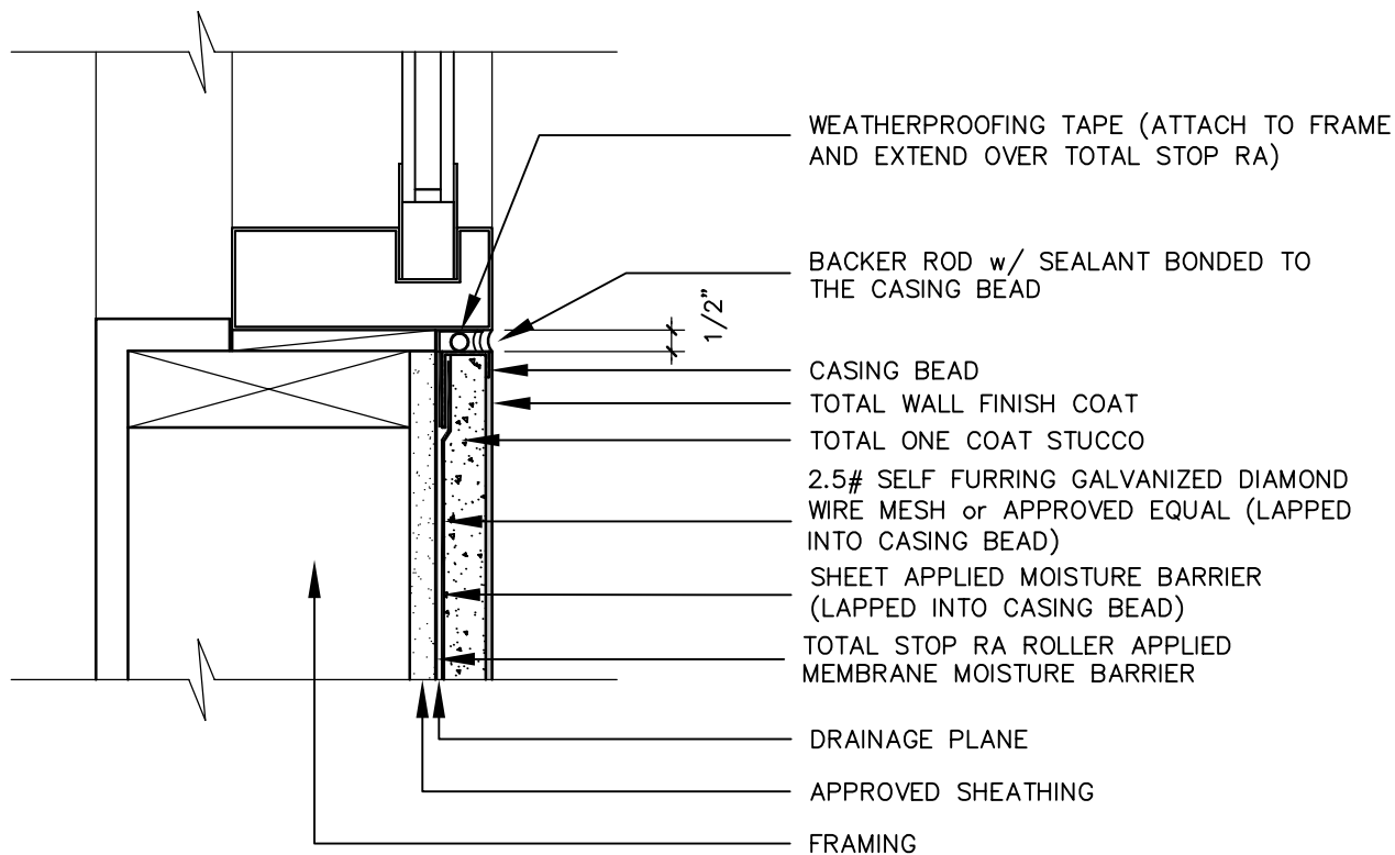
TODS-04.1 TYPICAL WINDOW SILL (FLUSH)
