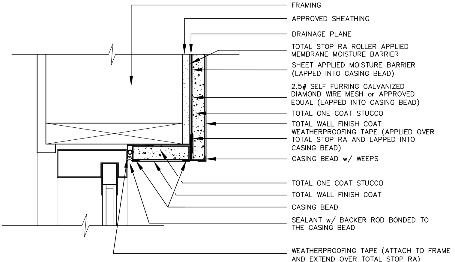
TODS-03.2 TYPICAL WINDOW/DOOR HEAD (RECESSED)
