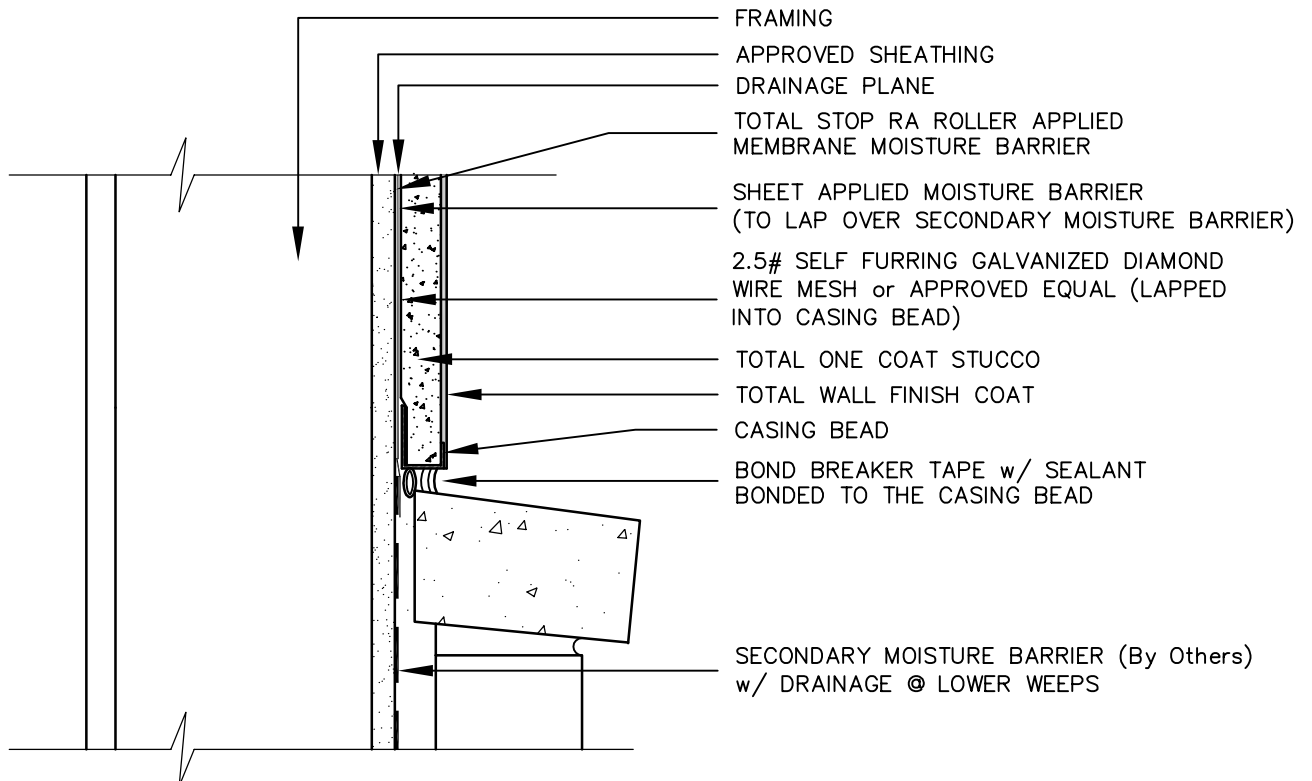
TODS-08.2 TYPICAL STUCCO @ MASONRY SILL
