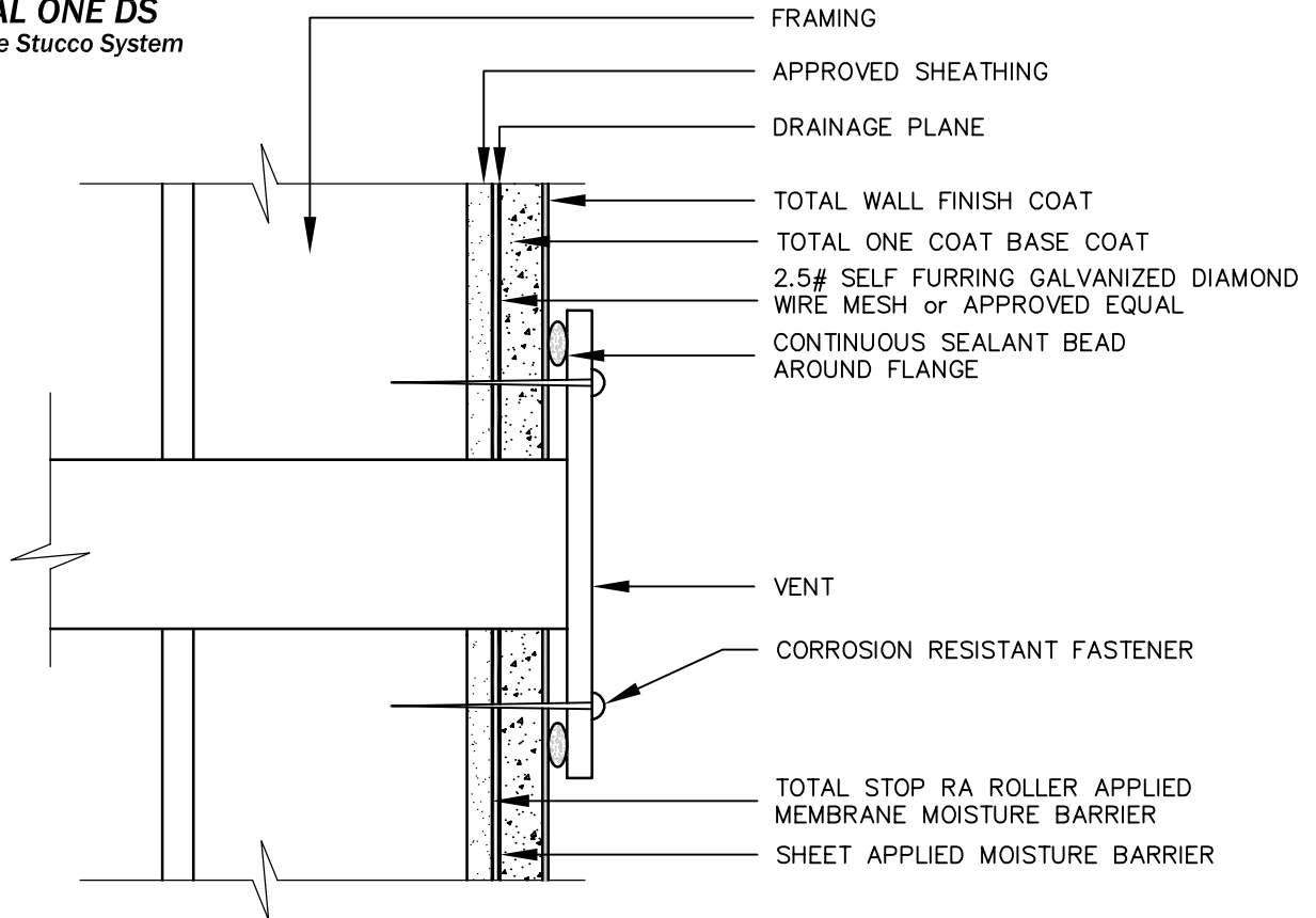
TODS-11 TYPICAL VENT ATTACHMENT
