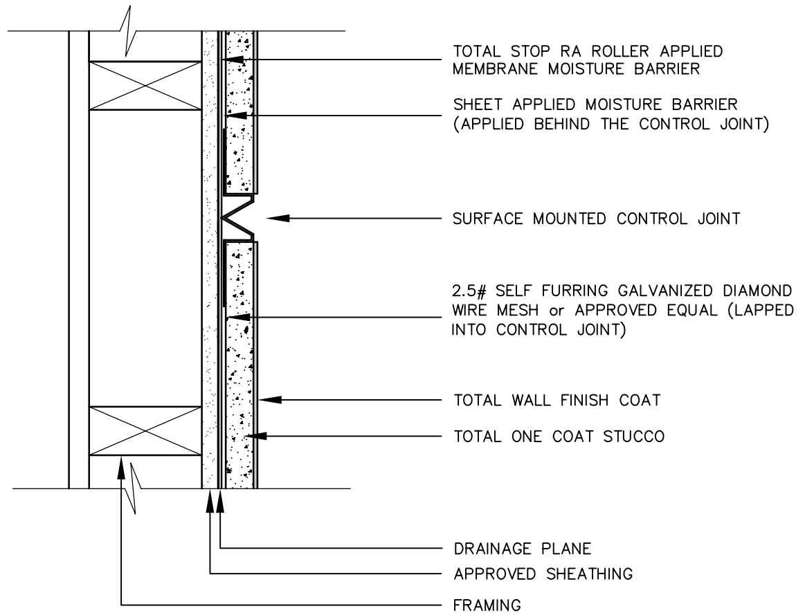
TODS-06.2 TYPICAL CONTROL JOINT
