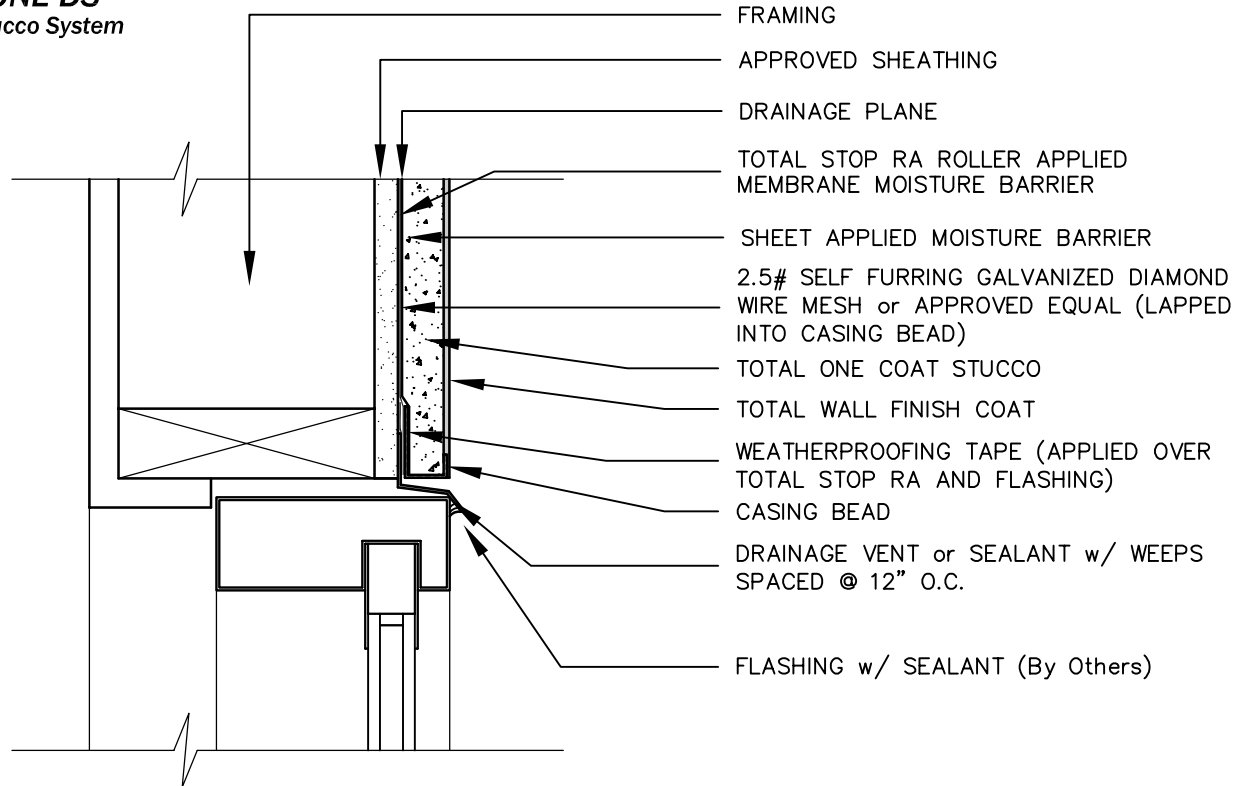
TODS-03.1 TYPICAL WINDOW/DOOR HEAD (FLUSH)
